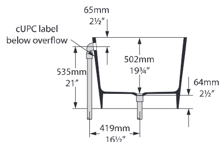
Section BB Shown with K51 waste kit
